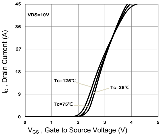
Figure 9. Transfer Characteristics
